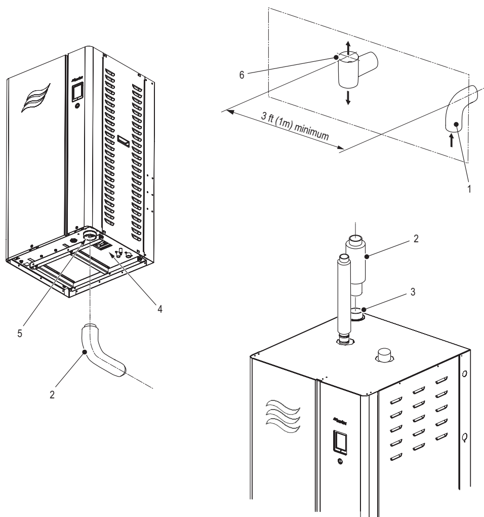
Figure 19: Nortec GS Sealed Combustion Connection
