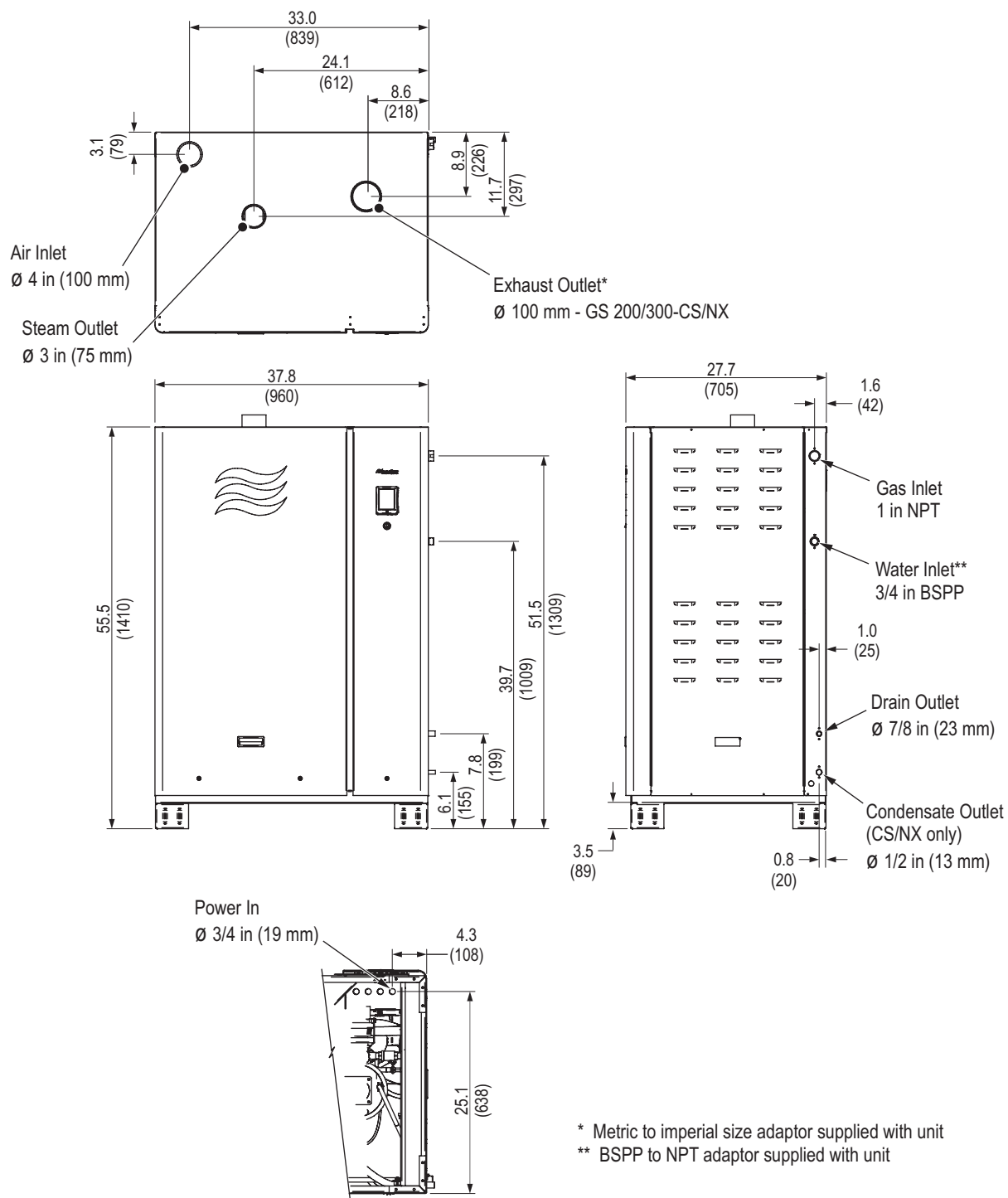
Figure 37: Nortec GS 200/300
