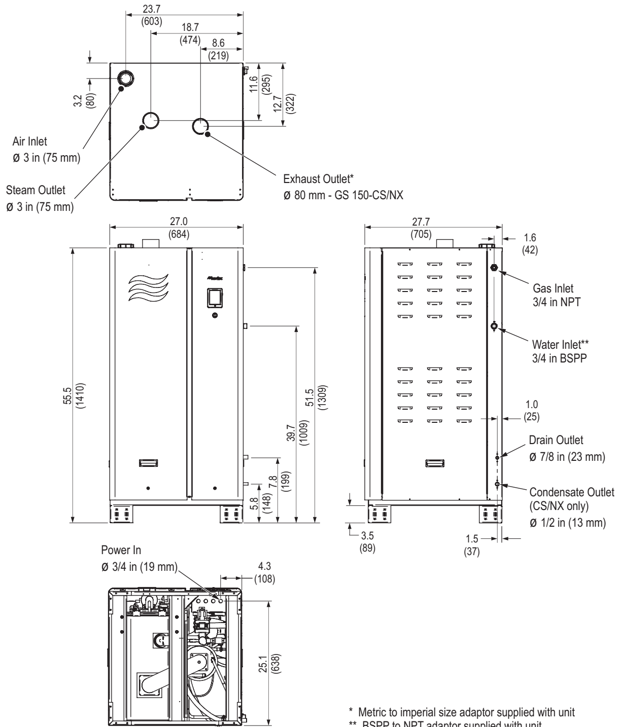
Figure 36: Nortec GS 150
