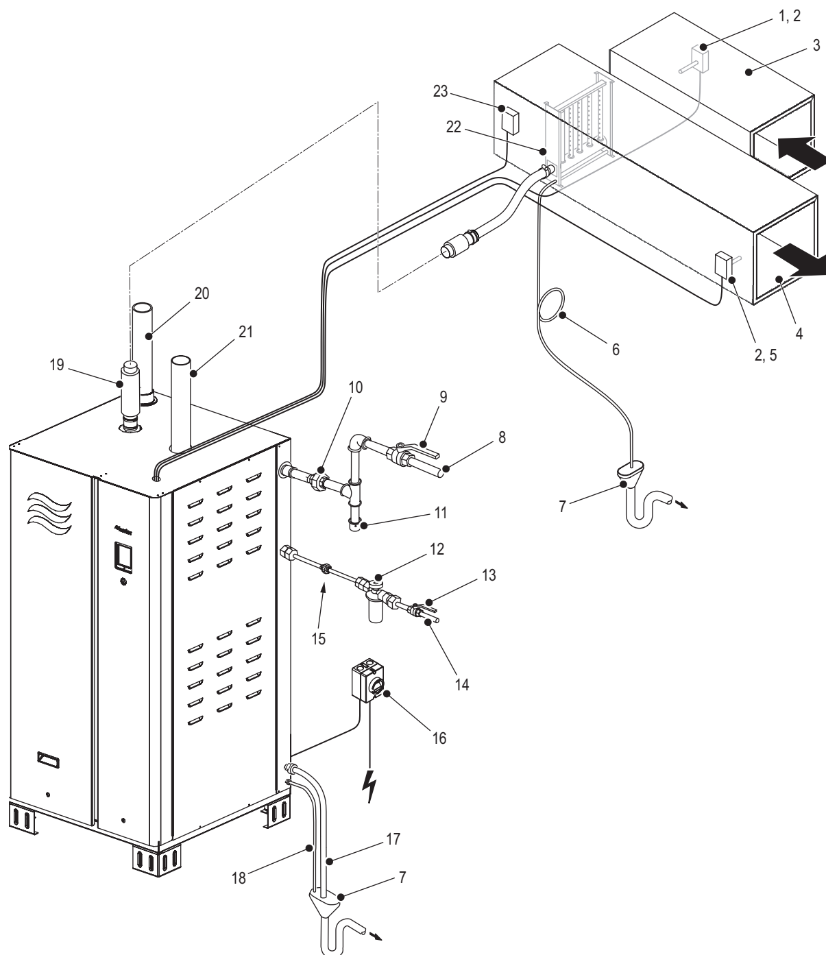
Figure 6: Installation Overview – Full-Size Units (GS 150 Shown)
