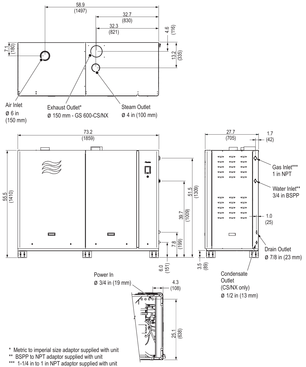
Figure 39: Nortec GS 600
