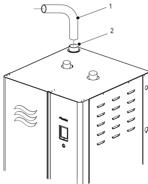
Figure 18: Space Air Installation – GS 150-650
